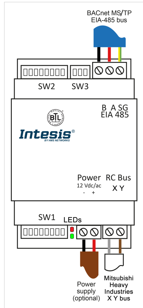
Figure 1. Wiring diagram (wire colors are indicative only)
